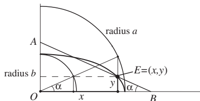
Figure 5. Angle of inclination of a trammel is also the eccentric angle of traced ellipse.
