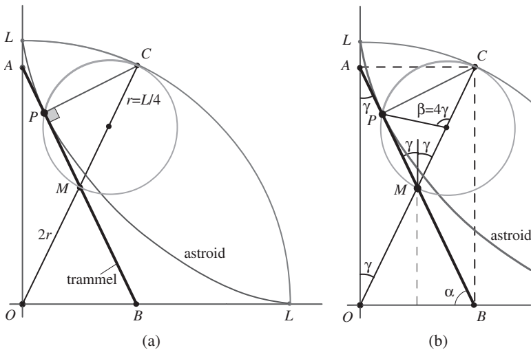
Figure 4. (a) Point P on the circle of radius L/4 traces an astroid as it rolls inside a circle of radius L . (b) Proof that AB has constant length equal to radius L .
