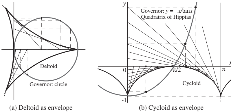
Figure 19. (a) A circular governor tangent to the y axis produces a deltoid as envelope. (b) Cycloid as envelope for quadratrix of Hippias as governor. Different branches of the quadratrix produce copies of the cycloid.
