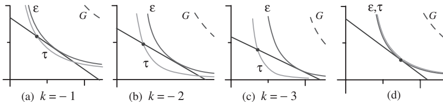
Figure 18. Special cases of Example 2 with negative k , and \lambda = 0.3 in (a)–(c).
