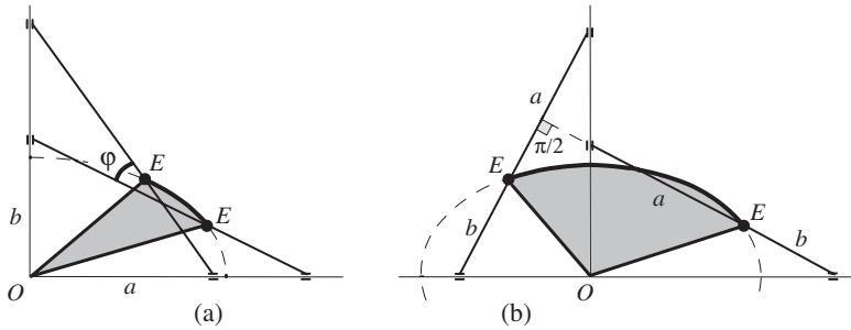
Figure 9. (a) Area of a general elliptical sector. (b) Special case with \varphi = \pi/2 .
