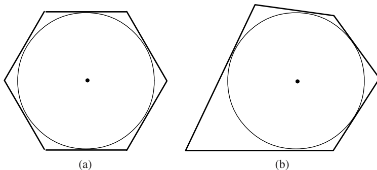
Figure 1. Example of circumgons: (a) a regular hexagon and (b) a nonregular pentagon.
