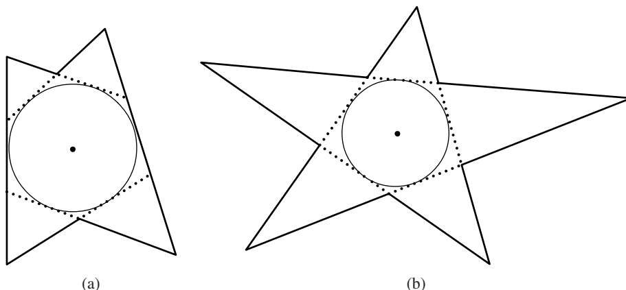
Figure 2. Some circumgonal regions: the area of each is its semiperimeter times its inradius.
