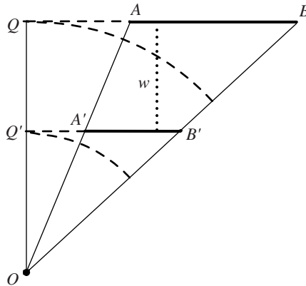
Figure 7. Illustrating the proof that every ring of constant width is a circumgonal ring.
